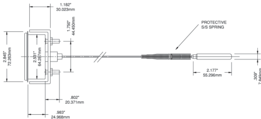
2.5" with U-Clamp
