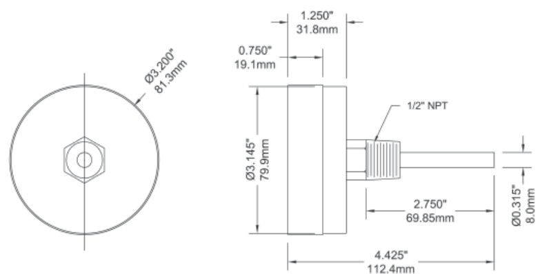
3" Back Connection
