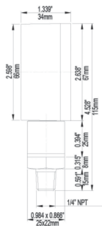
Without Rubber Boot
