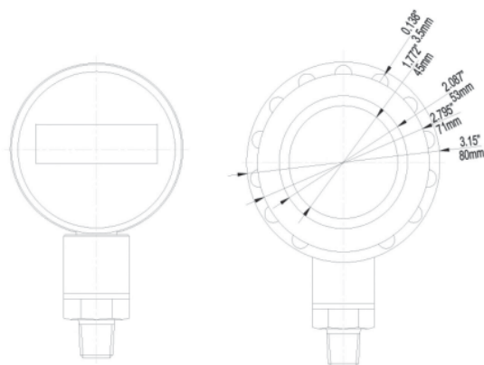
Without Rubber Boot
