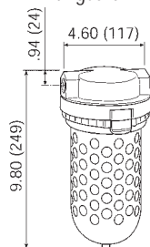
with guard
